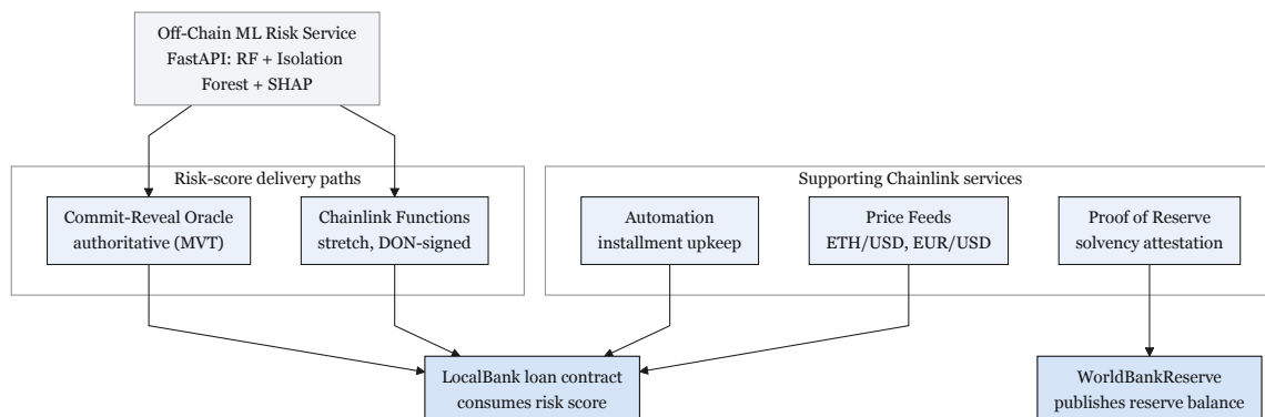
Figure 3.4: Oracle architecture
