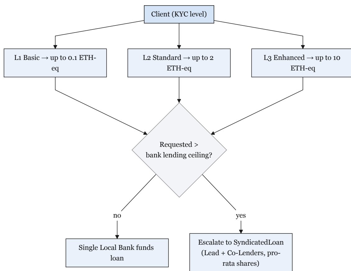
Figure 3.15: Client limits and bank-level syndication
