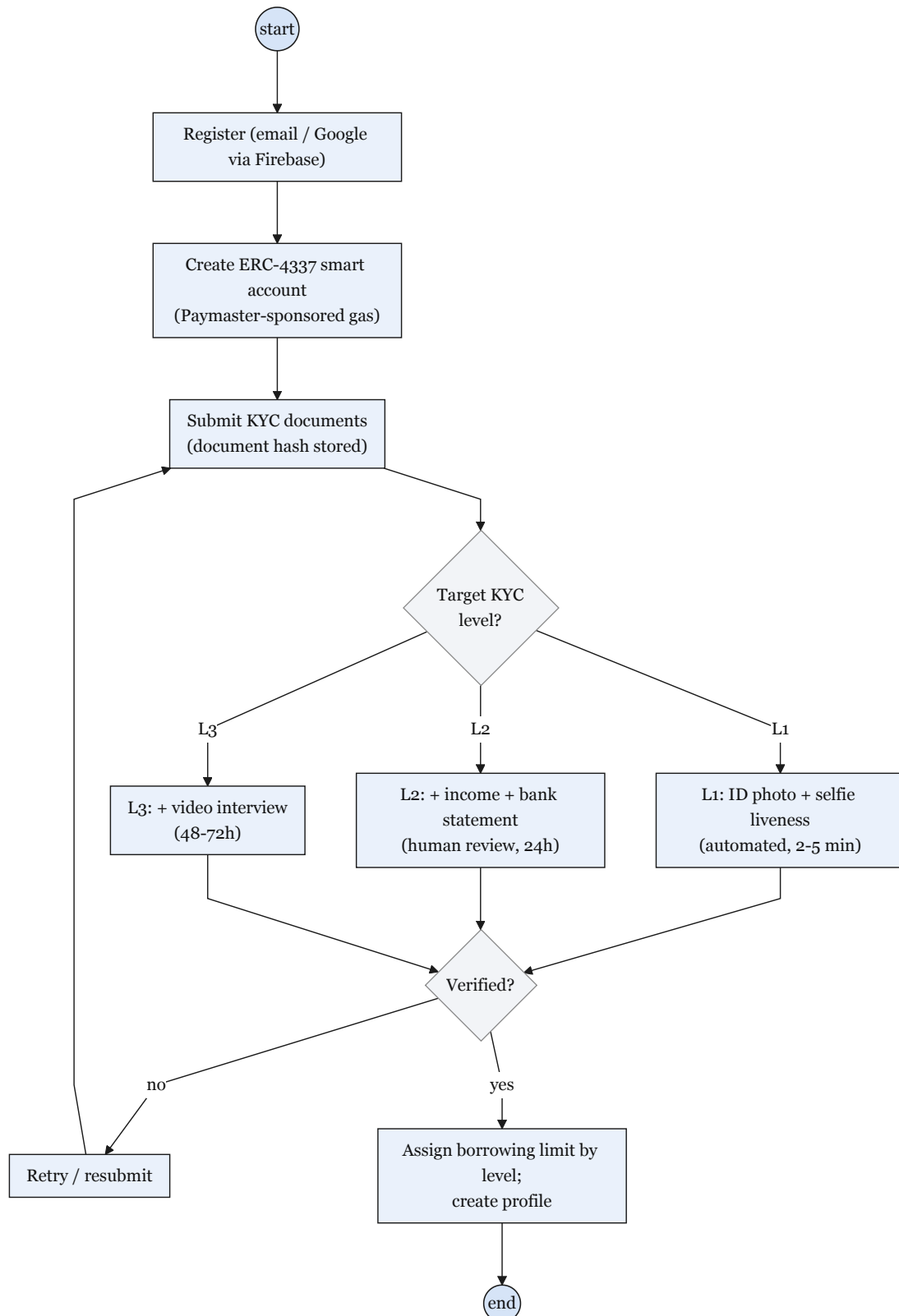
Figure 3.25: Retail onboarding and identity activity flow
