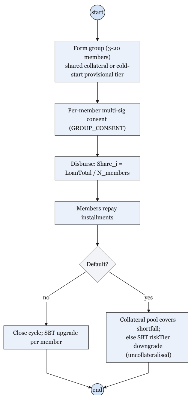
Figure 3.34: Solidarity group lending lifecycle
