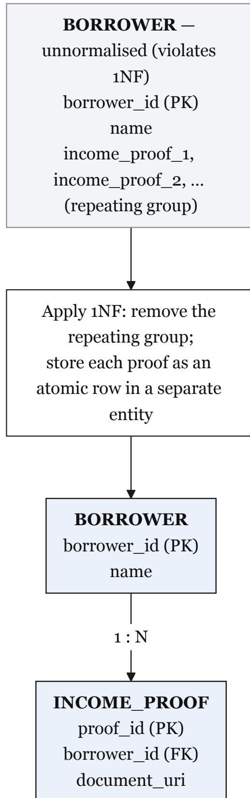
Figure 3.9: First normal form (1NF) demonstration
