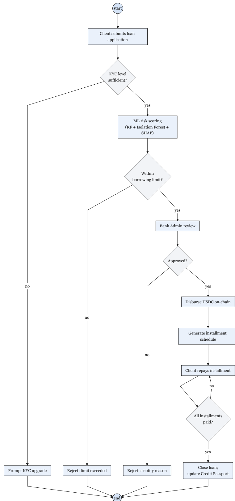
Figure 3.24: USDC loan lifecycle activity flow
