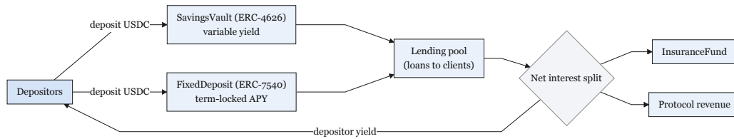
Figure 3.20: SavingsVault and FixedDeposit closed loop
