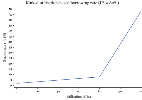
Figure 3.18: Kinked utilization-based borrowing rate
