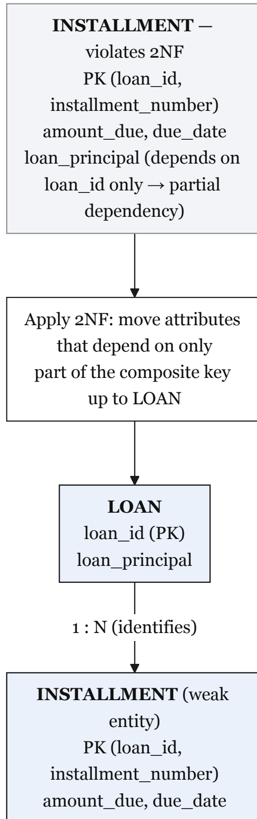
Figure 3.10: Second normal form (2NF) demonstration
