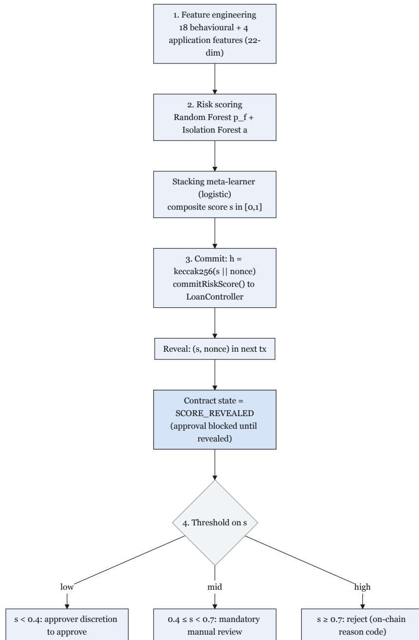
Figure 4.2: ML oracle commit–reveal gate
