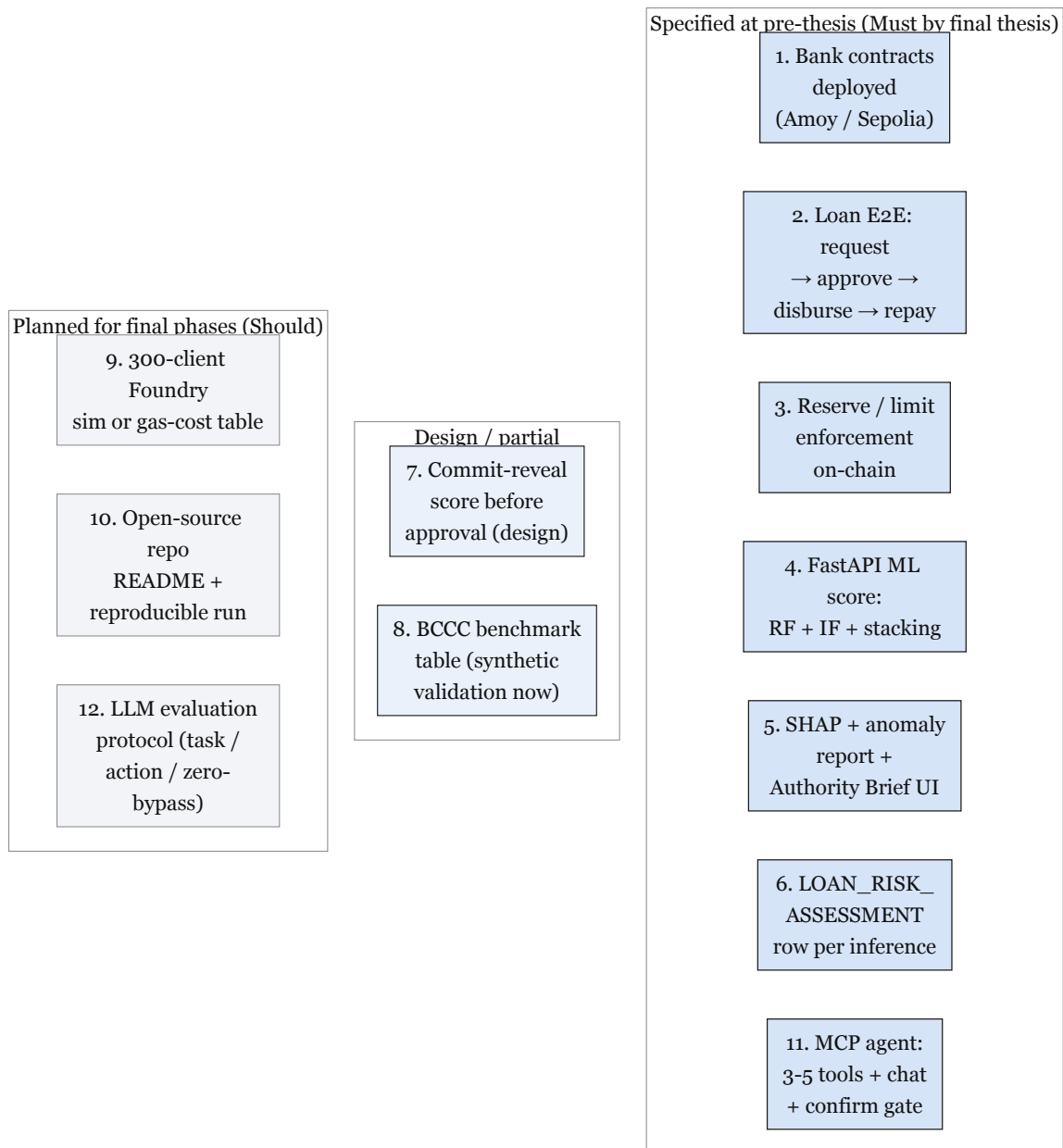
Figure 4.1: MVT deliverable status at pre-thesis
