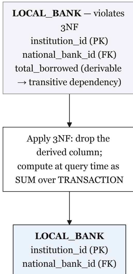
Figure 3.11: Third normal form (3NF) demonstration
