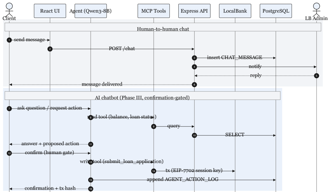
Figure 3.31: Sequence diagrams
