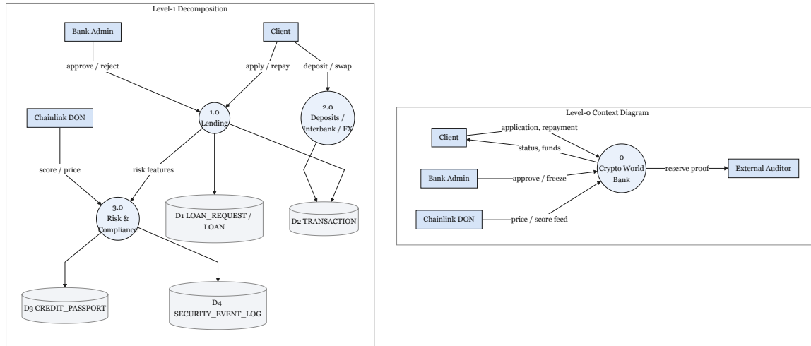
Figure 3.27: Data-flow diagrams
