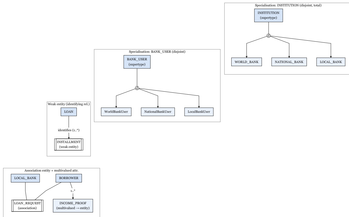
Figure 3.8: Enhanced EER model
