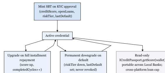
Figure 3.21: On-chain Credit Passport SBT lifecycle
