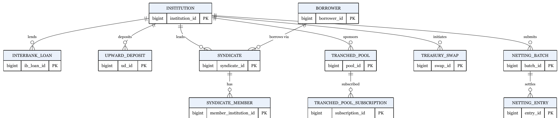
Figure 3.7: Extended ERD: multi-entity and cross-tier operational entities (crow's-foot; PK shown, full attributes in Table 3.17).
