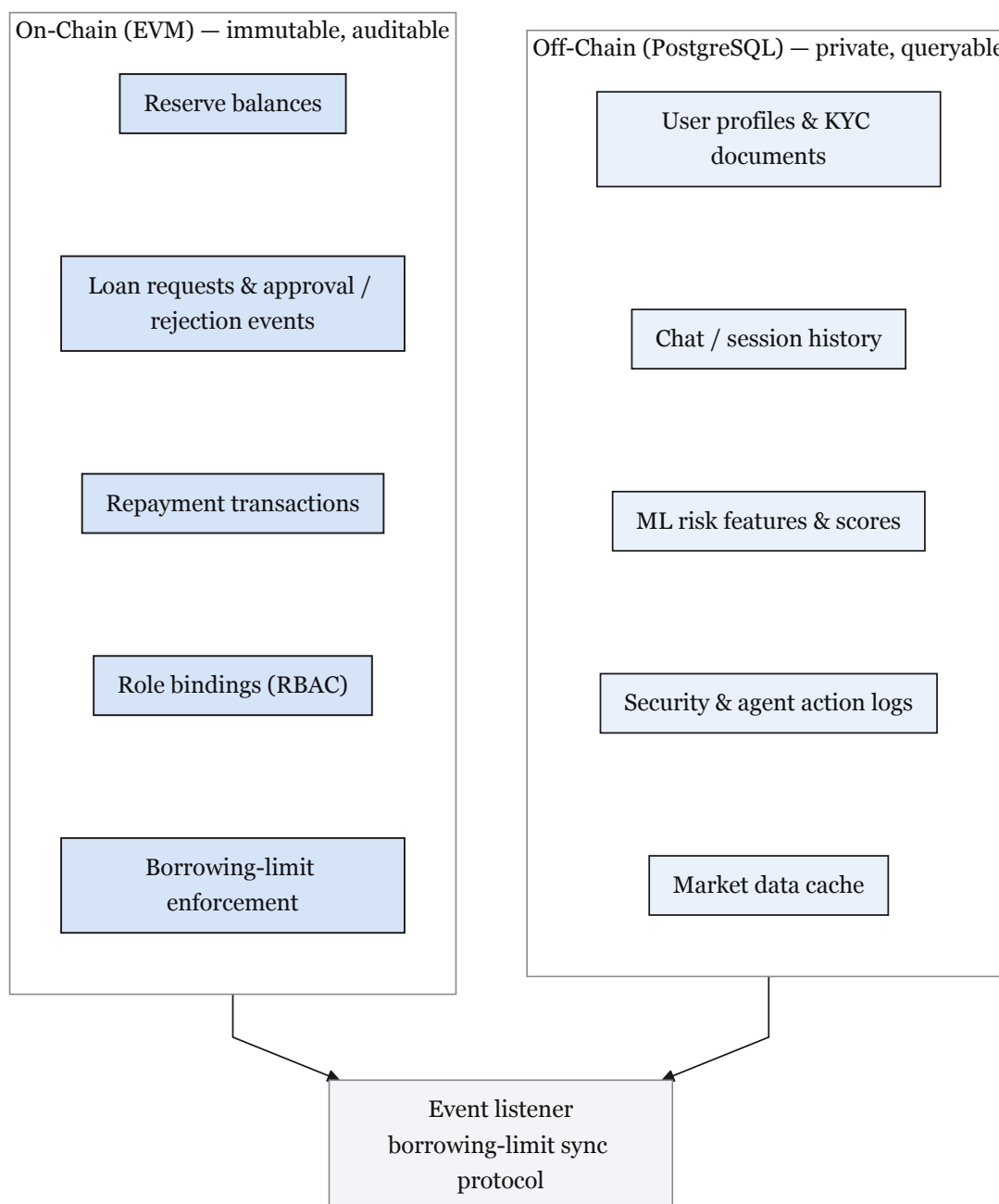
Figure 3.13: On-chain versus off-chain data partitioning
