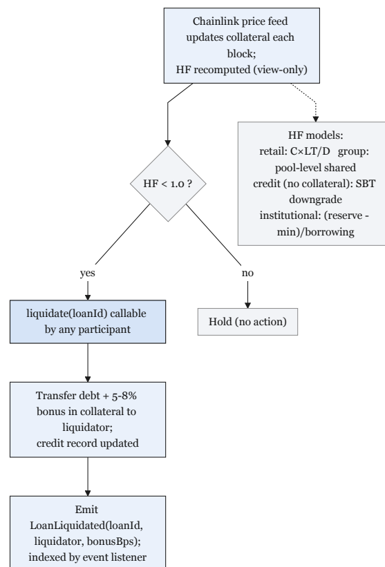
Figure 3.19: LiquidationEngine tier models and lifecycle
