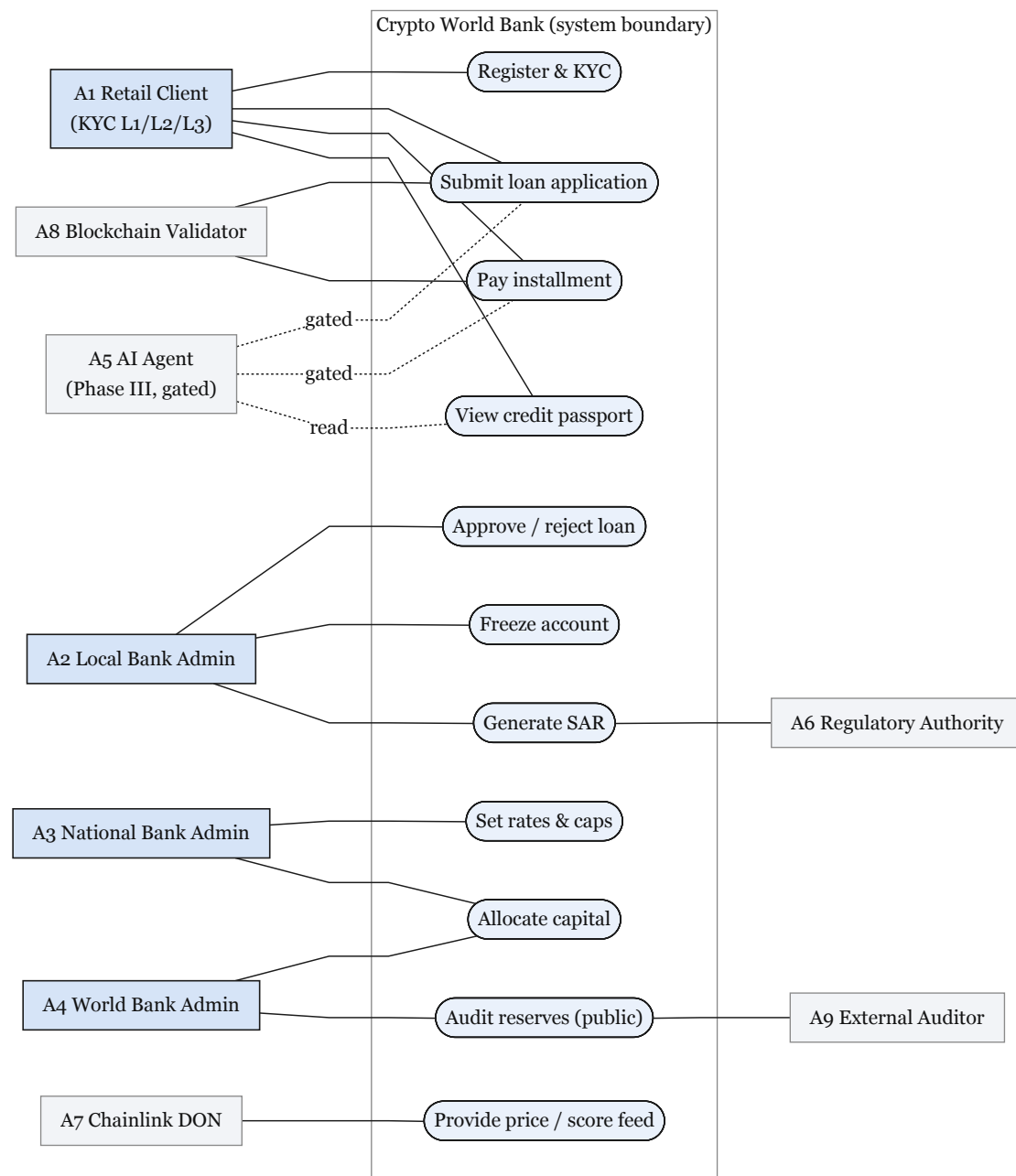
Figure 3.23: Use-case diagram (nine-actor taxonomy)
