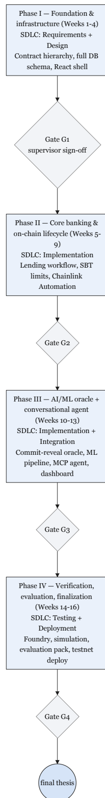
Figure 4.3: Four-phase roadmap with SDLC mapping and progress
