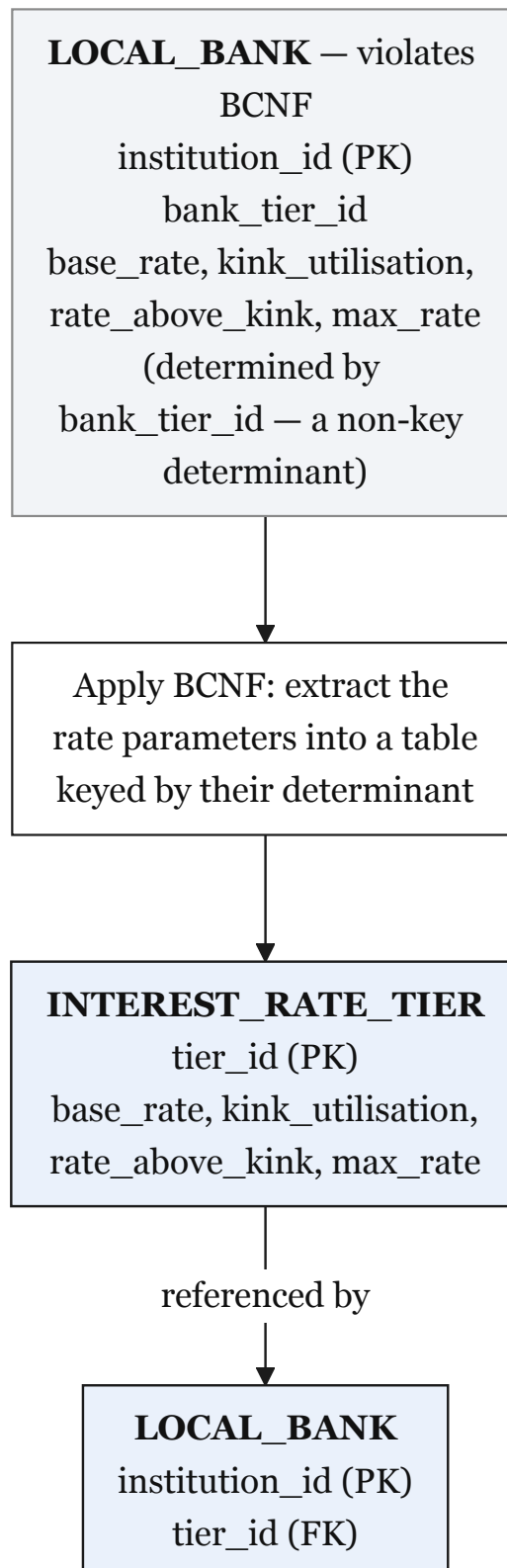
Figure 3.12: BCNF verification on INTEREST_RATE_TIER
