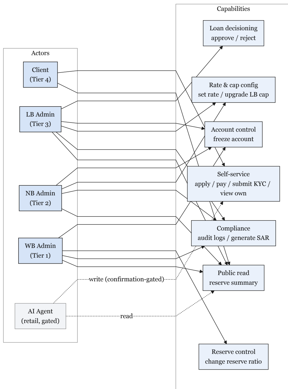
Figure 3.14: Actor permission matrix (primary actions)
